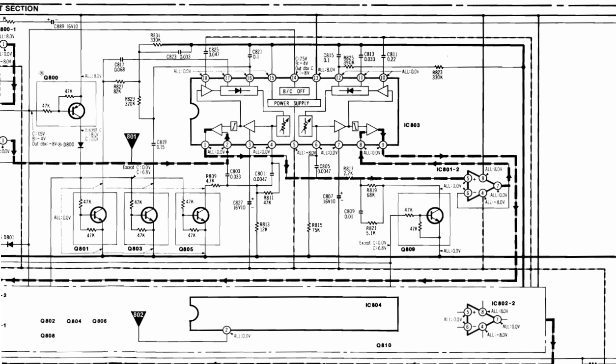
D800, 801 [MA150] Q800 [UN4113] Q801~810 [UN4213] IC803, 804 [NE651N] IC801~802 [M5218L]
