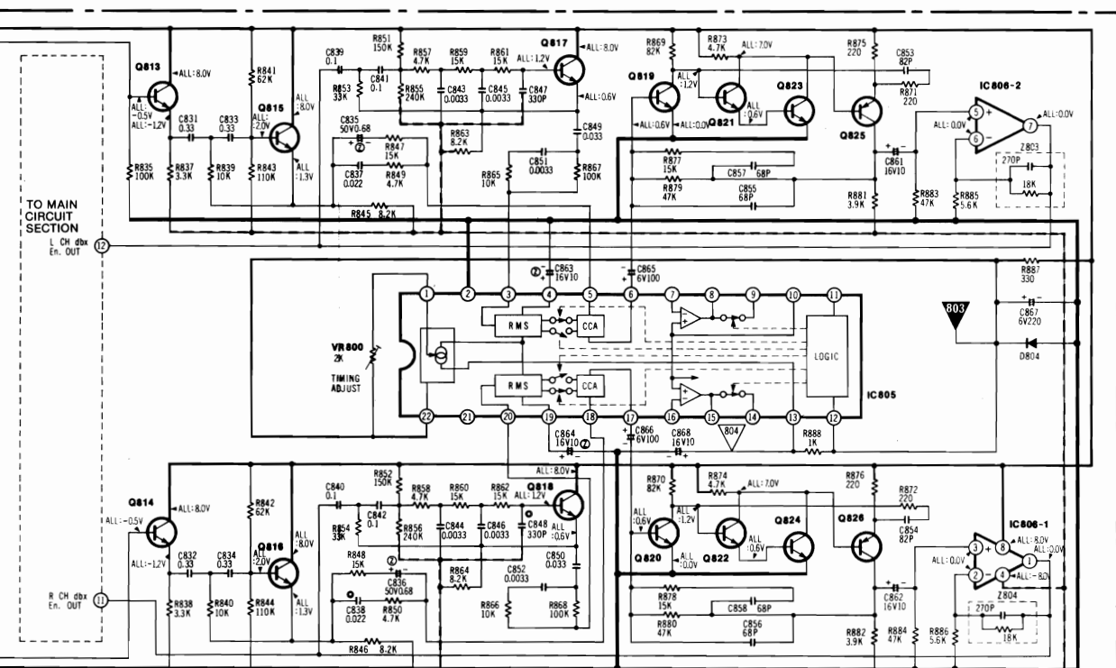
Q813~816, 821~824 [2SC2603E] [2SC2603] Q817, 818 [2SD1011S] [2SD1011] Q819, 820 [2SD661R] [2SD661] IC805 [AN6291] Q825, 826 [2SA1115E] [2SA1115] IC806 [M5218L] D804 [MA1051M] [MA1051]
