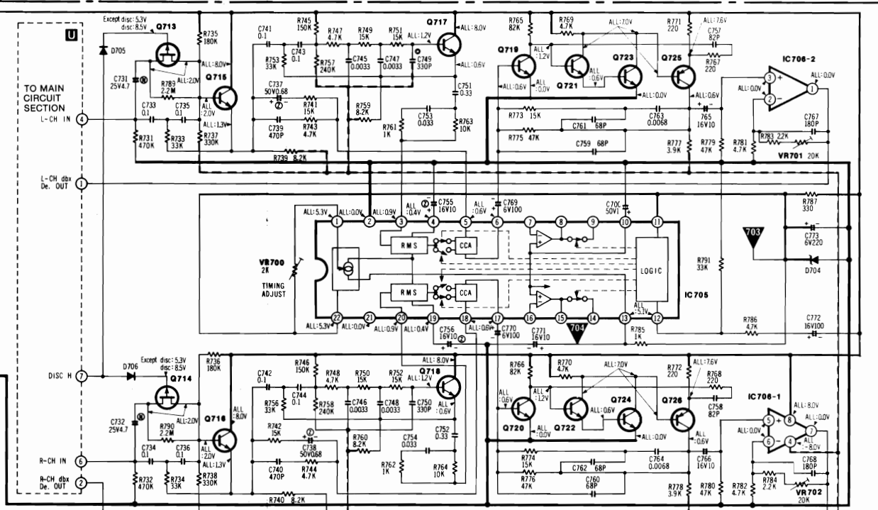
Q715, 716, 721~724 [2SC2603E] [2SC2603] Q717, 718 [2SD1011S] [2SD1011] Q719, 720 [2SD661R] [2SD661] IC705 [AN6291] Q725, 726 [2SA1115E] [2SA1115] IC706 [M5218L] D704 [MA1051M] [MA1051]
