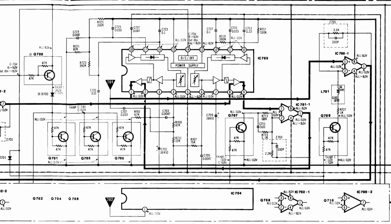
D700, 701 [MA150] Q700 [UN4113] Q701~710 [UN4213] IC703, 704 [NE651N] IC700~702 [M5218L]
